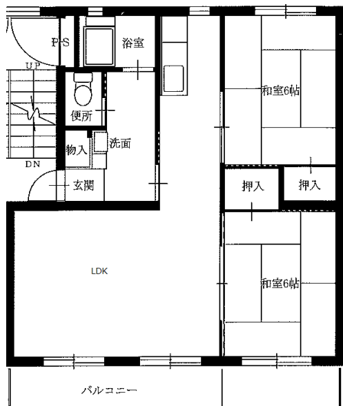
2LDK-A(2-11)
